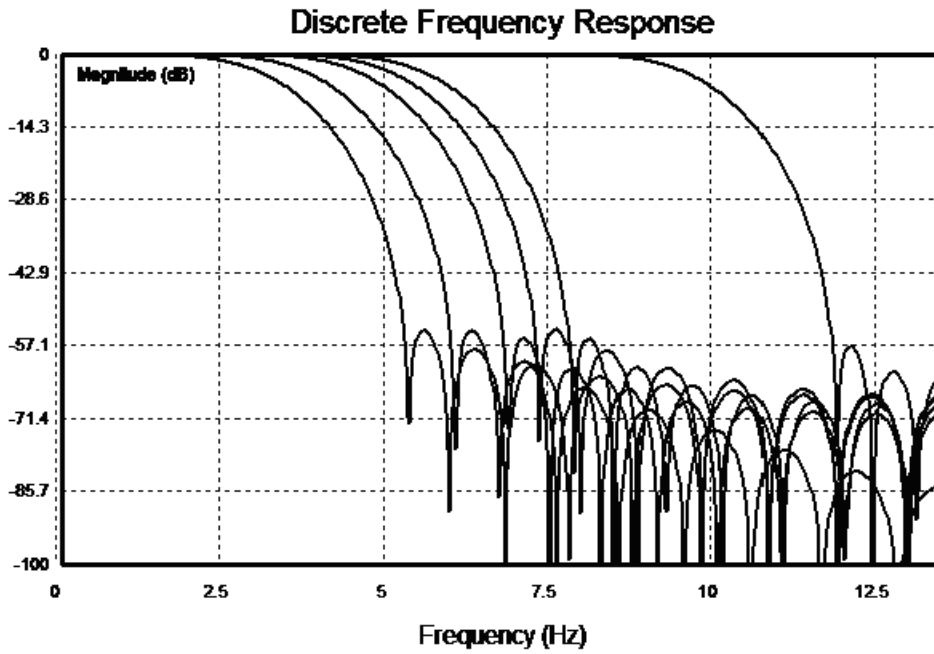
Figure 7. Luma filter
