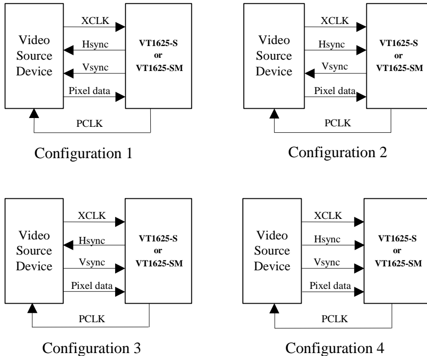
Figure 3. Master Clock Mode 1
