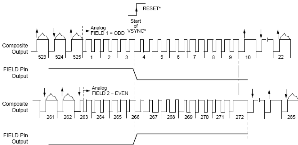
Figure 6. Field Output
